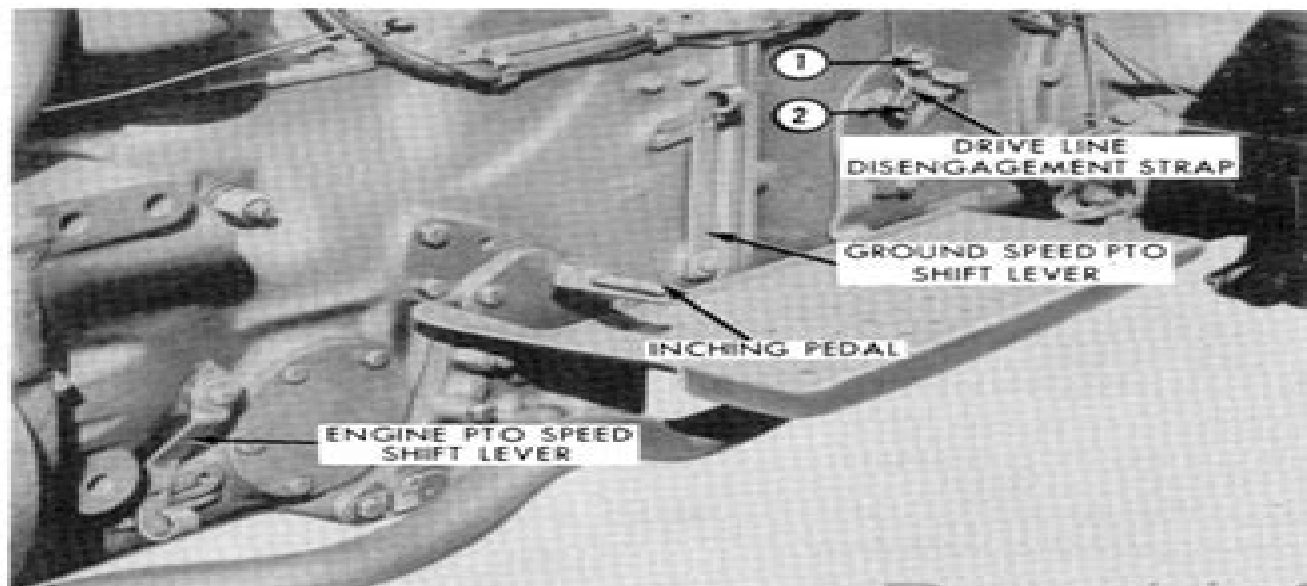
Figure 6 Controls on the Select-O-Speed Transmission
